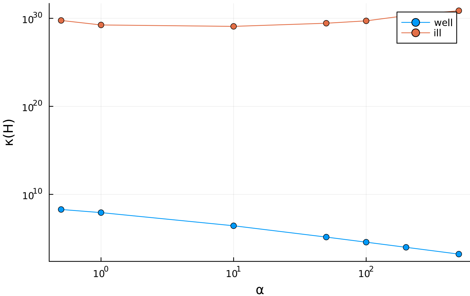
conditioning vs \alpha
